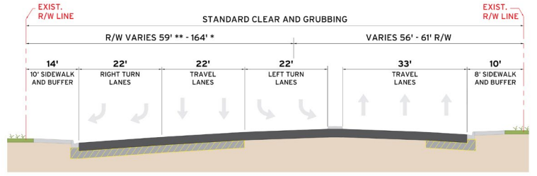
TYPICAL SECTION | SIMPSON ROAD
