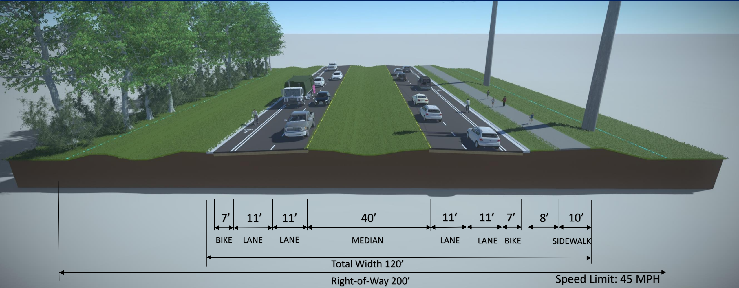
Typical Section
