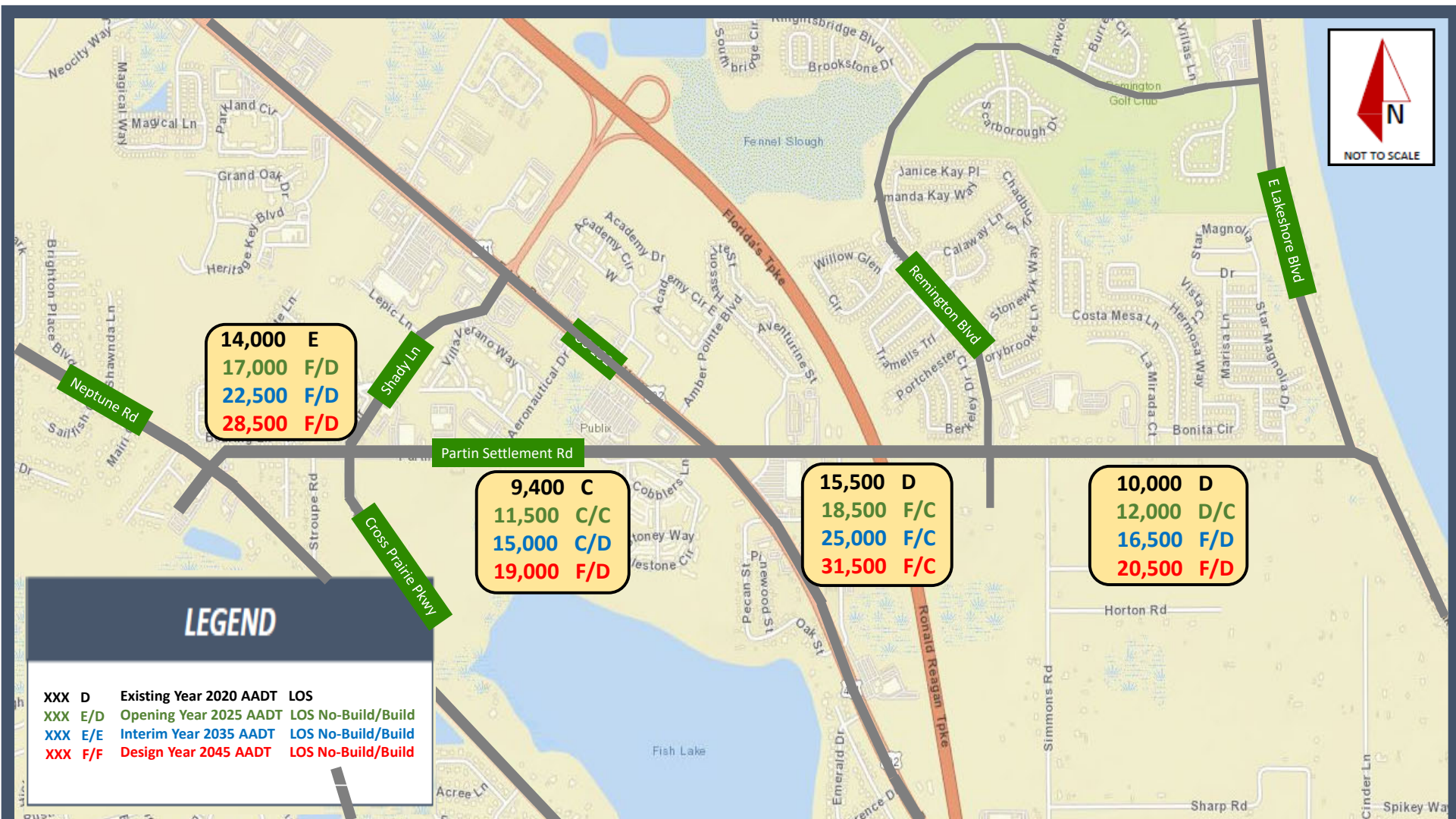
Existing Year 2020, Opening Year 2025, Interim Year 2035 and Design Year 2045 AADT and No-Build/Build Level of Service (LOS) Partin Settlement Road PTAR
