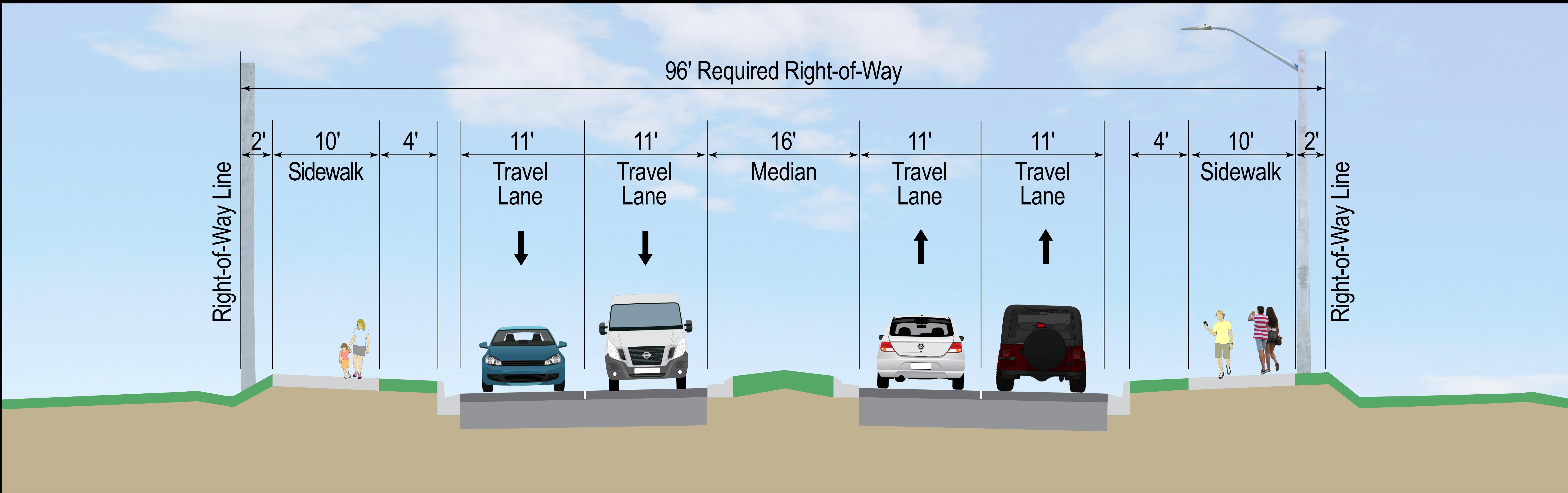
Partin Settlement Road Four-Lane Divided Section
