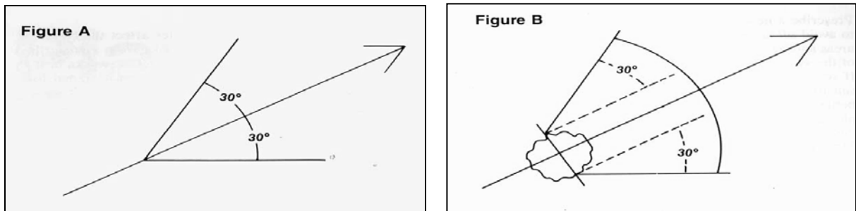
Fig. 3 Predicted footprint of smoke plume.
